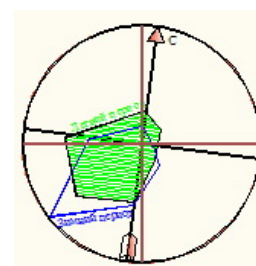
Figure 1 Wind rose from Kargalinsk weather station 92km SW of the mine showing prevalence of SW winds in winter (blue line) and W, SW and S winds in summer (green area).
