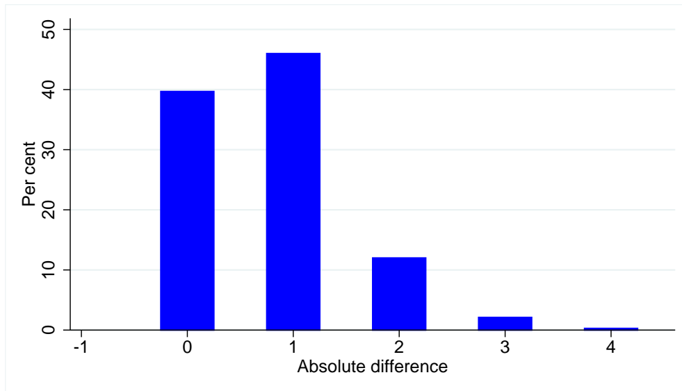
Chart A1: Histogram of the absolute difference in responses
