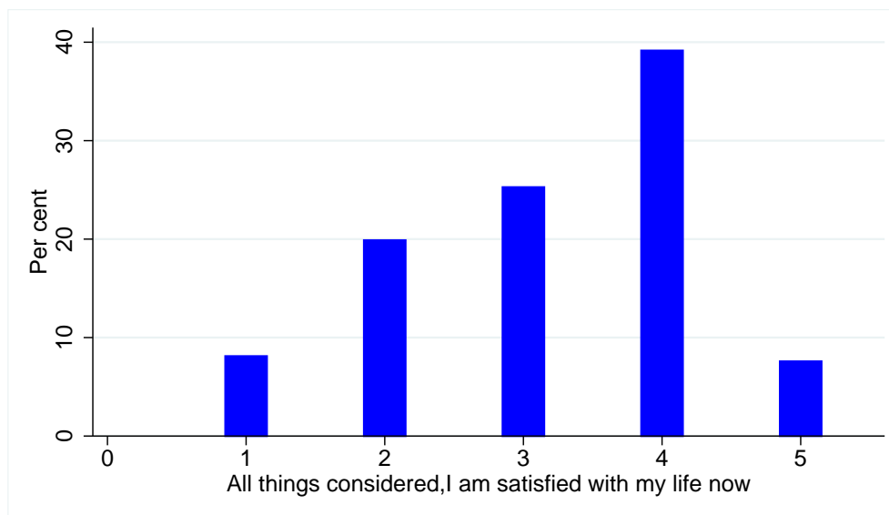
Chart 2: Distribution of responses – second life satisfaction question
