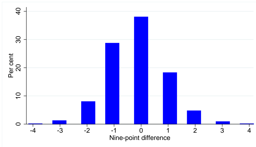
Chart 3: Histogram of the nine-point difference in responses
