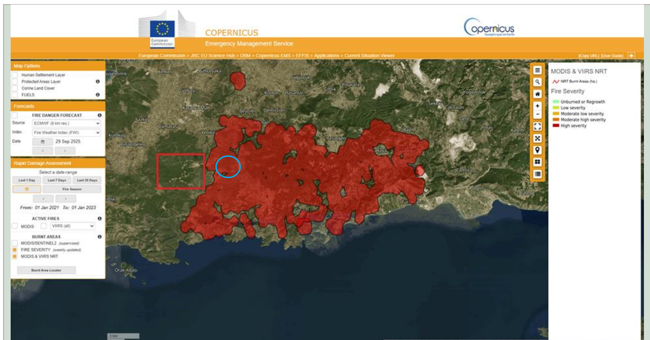
FIGURE 3-3 BURNT AREA MAP (COPERNICUS EMS)
