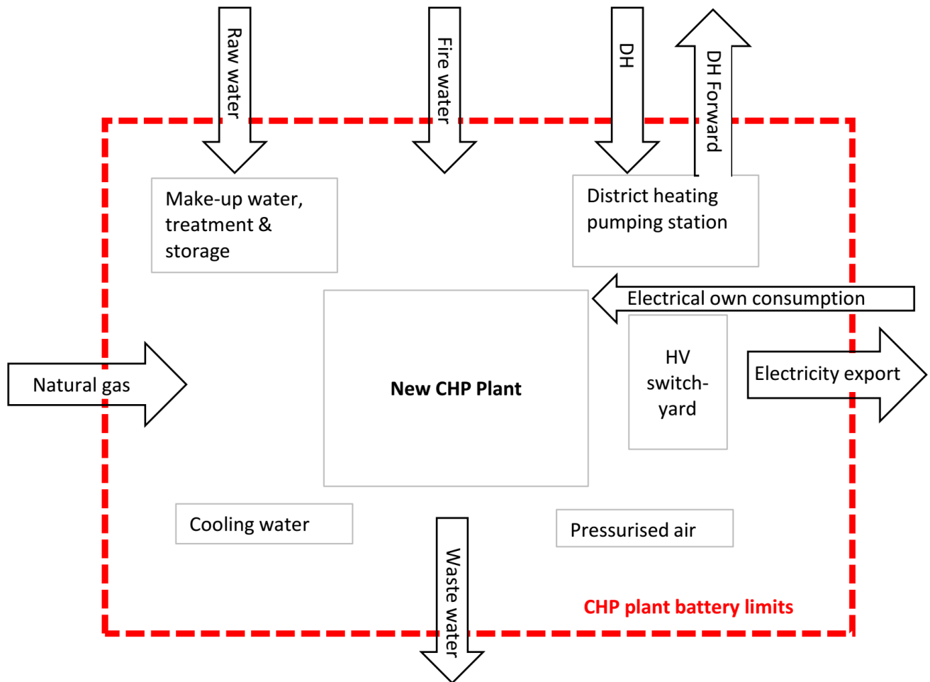
Figure 1 New CHP battery limit diagram.
